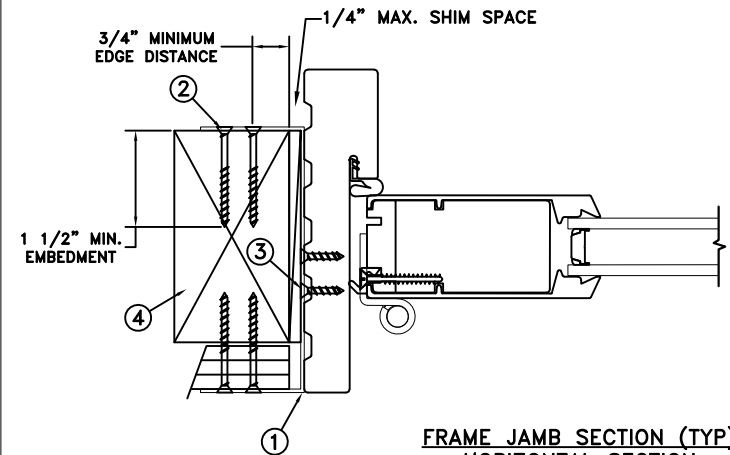
FRAME SECTION (TYP) VERTICAL SECTION
